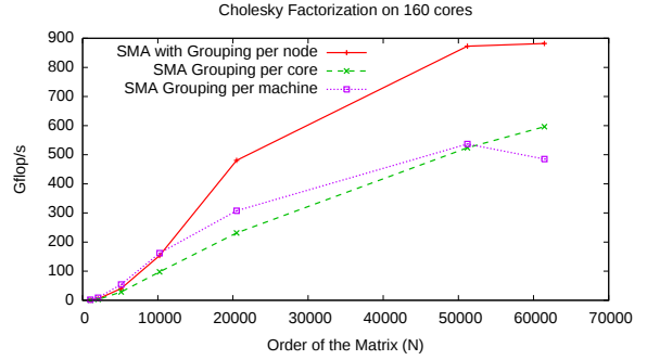
Figure 3: Comparison of different grouping strategies for the Cholesky factorization on a 160 cores, 20 nodes machine. Grouping per machine, node and core respectively corresponding to G=1 , 20 and 160.
