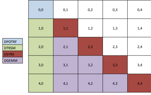
(a) Kernels modifying each tile for k = 1 and T = 5
