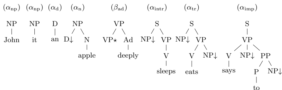
Fig. 2: A toy LTAG for English.
