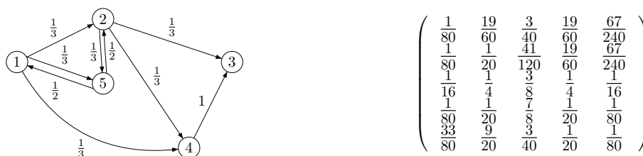
Fig. 3. (a) P , a Markov chain model of a subgraph of the World Wide Web and (b) the transformed irreducible and aperiodic chain P' in matrix form
