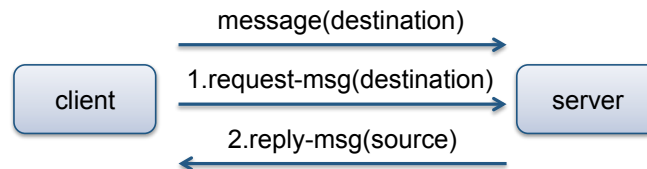
Figure 3.4: CS space and time coupling semantics
