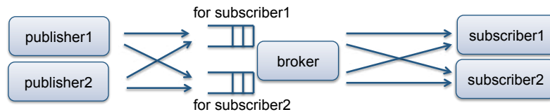
Figure 3.12: PS concurrency semantics
