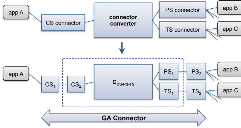
Figure 3.27: Application of the conversion method to GA
