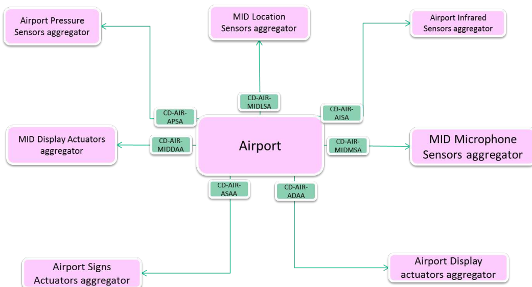
Figure 4.17: (b) Architecture of the airport use case
