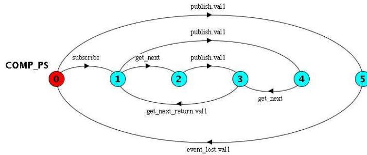
Figure 3.33: PS connector constrained by component port
