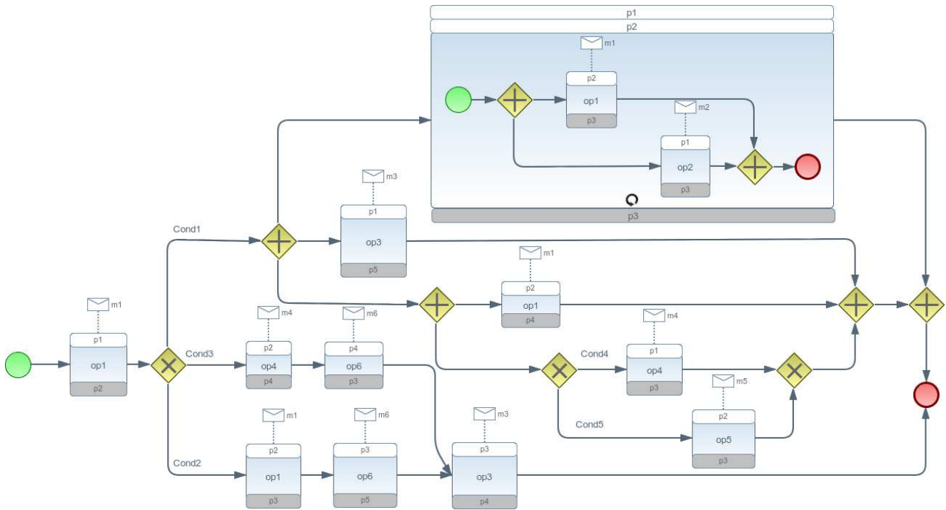
Figure 4.7: BPMN2 choreography diagram example
