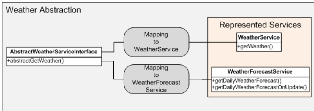
Figure 2.4: A functional abstraction for weather services.
