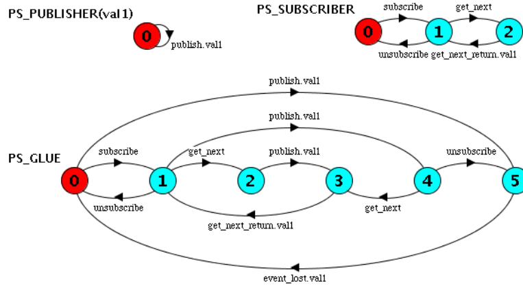
Figure 3.15: PS behavioral semantics
