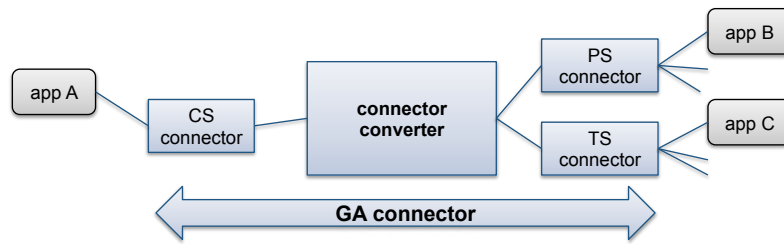
Figure 3.2: GA-based connector interoperability
