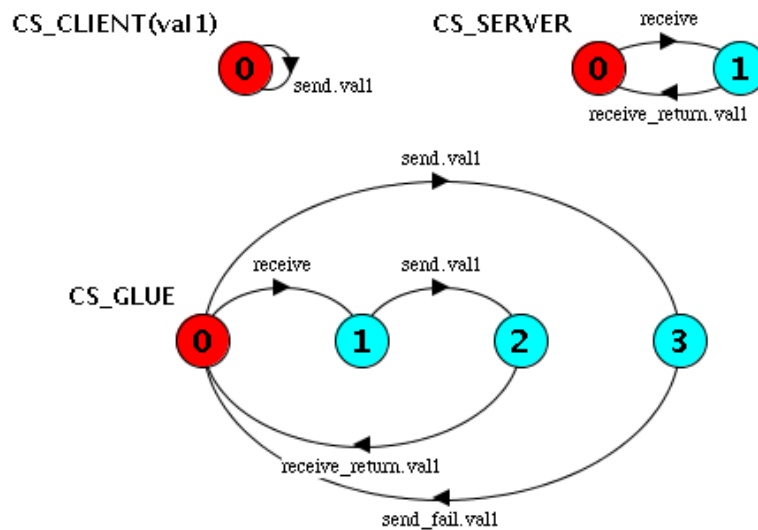
Figure 3.8: CS behavioral semantics for one-way interaction
