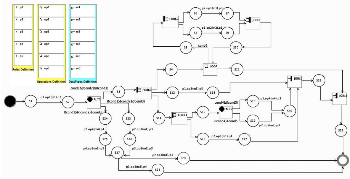
Figure 4.8: CLTS derived from the BPMN2 choreography diagram in Figure 4.7
