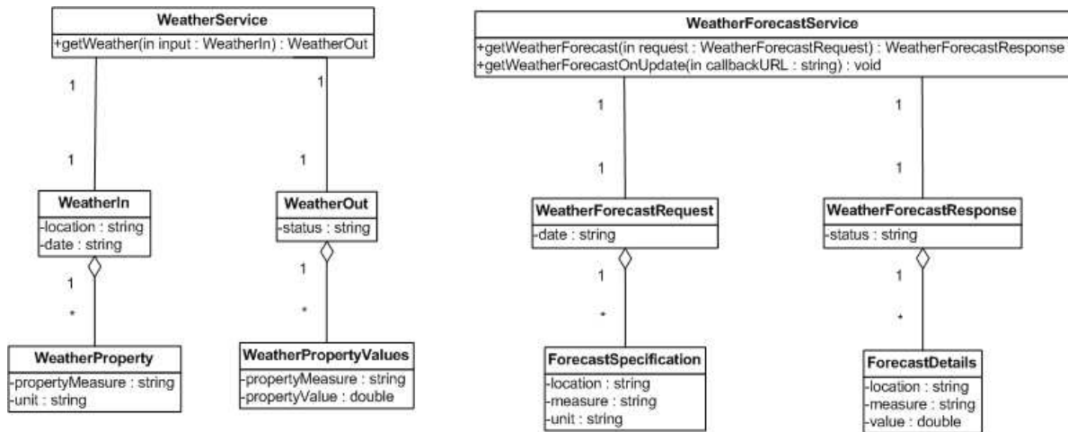
Figure 2.1: Weather services for the passenger friendly airport use case.
