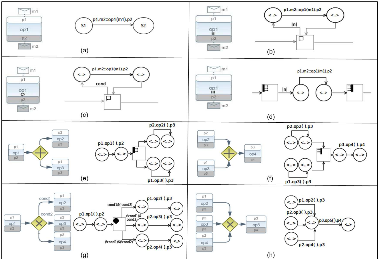
Figure 4.5: From BPMN2 choreography diagram to CLTS
