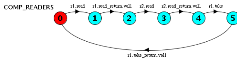
Figure 3.32: TS component port refining two reader roles
