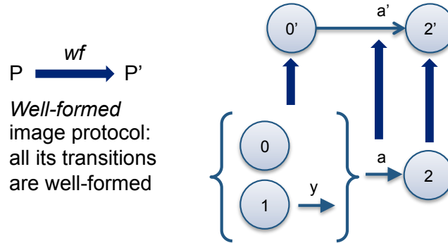
Figure 3.24: Well-formed image protocol
