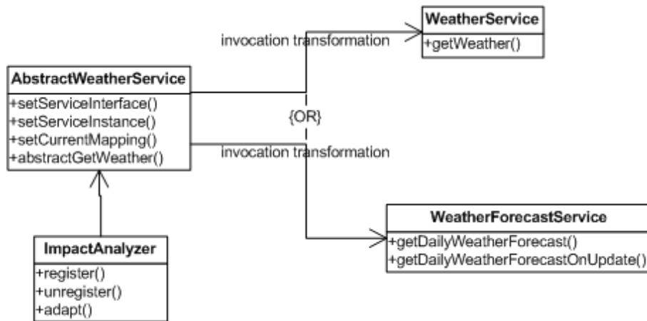
Figure 2.13: A functional abstraction service for the weather services.
