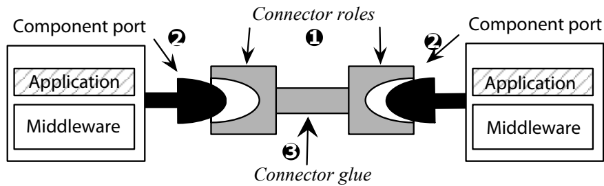
Figure 3.1: Components & Connector
