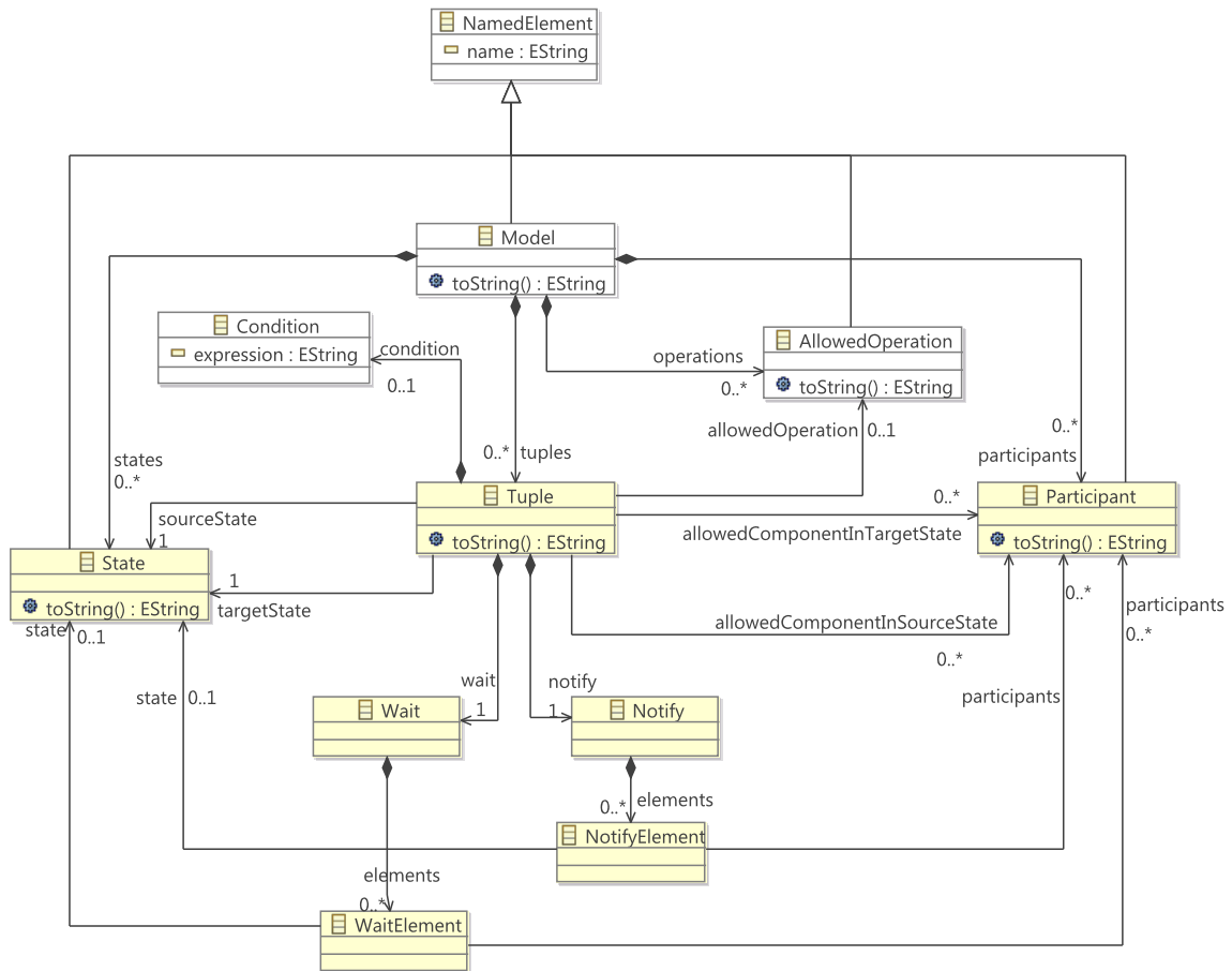
Figure 4.4: Coord metamodel
