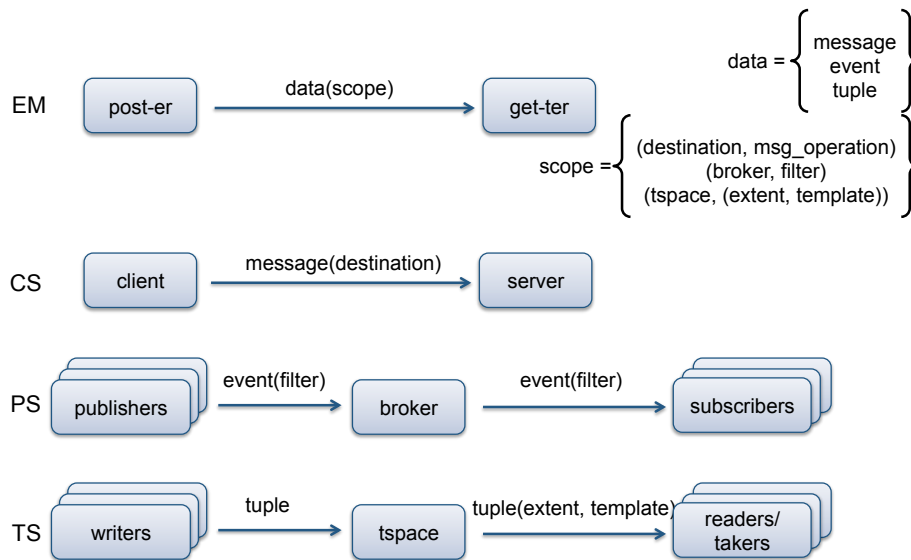
Figure 3.22: GA space coupling semantics wrt. CS, PS, TS space coupling semantics
