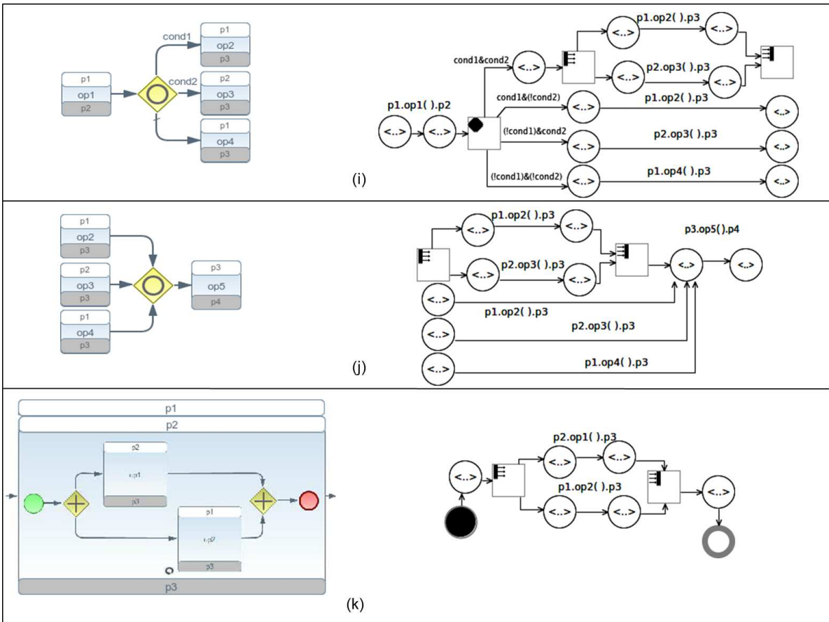
Figure 4.6: From BPMN2 choreography diagram to CLTS (Cont'd)
