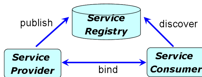
Figure 1.1: Service-oriented interaction pattern
