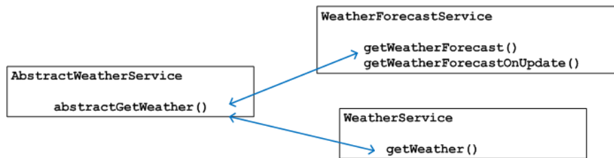
Figure 2.5: Operation mappings for the weather service abstraction.
