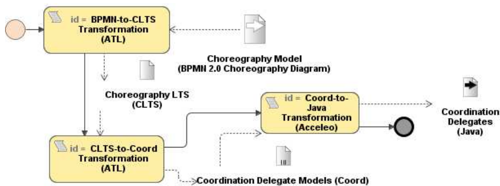
Figure 4.2: CHOReOS synthesis process
