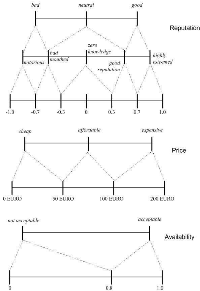
Figure 2.9: Domain hierarchies for reputation, price and availability
