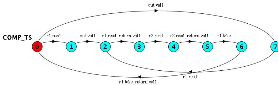
Figure 3.34: TS connector constrained by component port
