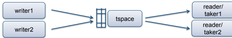
Figure 3.18: TS concurrency semantics
