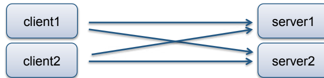
Figure 3.5: CS concurrency semantics
