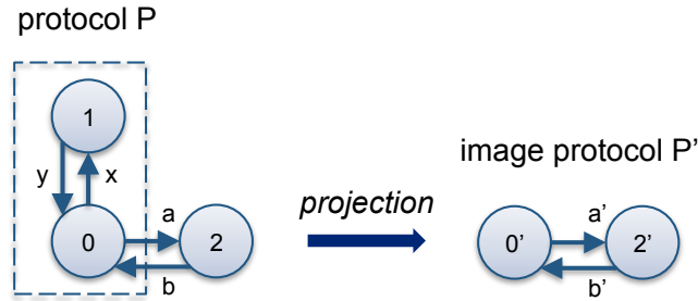
Figure 3.23: Protocol projection
