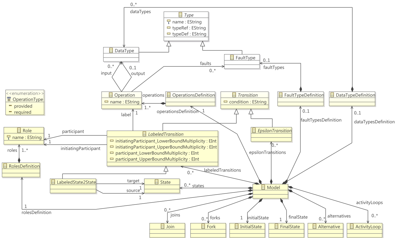
Figure 4.3: CLTS metamodel
