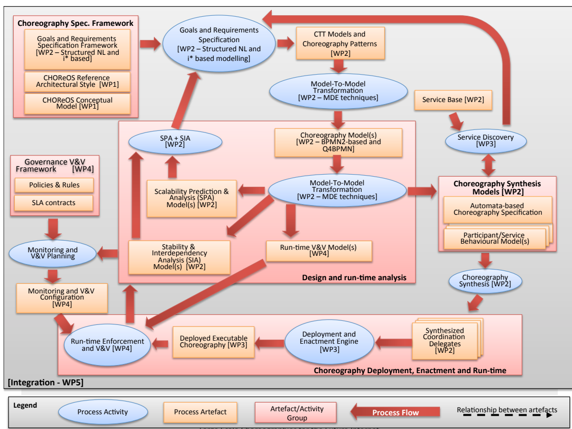
Figure 5.1: The CHOReOS development process
