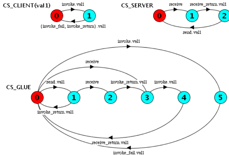
Figure 3.9: CS behavioral semantics for two-way interaction
