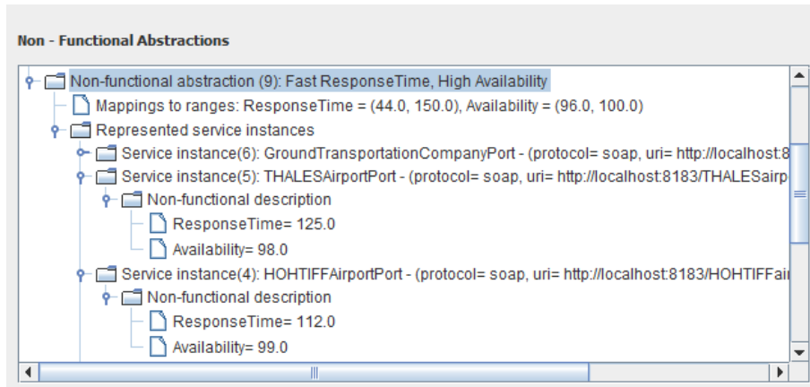
Figure 2.10: Non-functional abstraction representation in the AoSBM.
