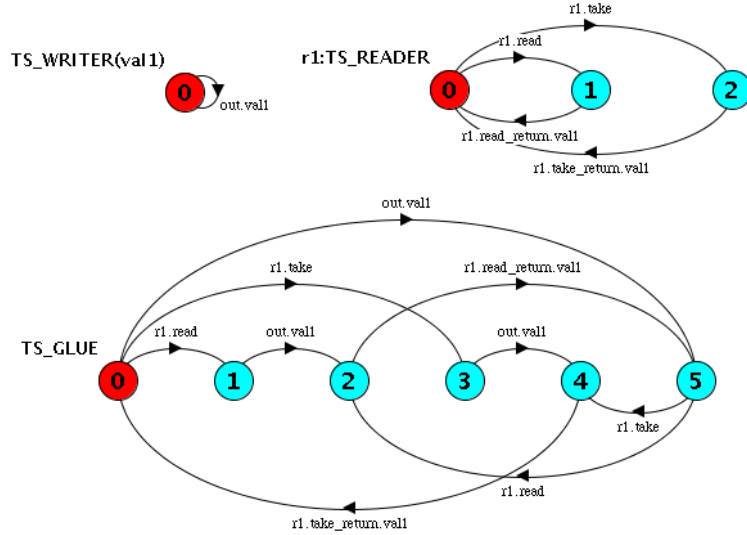
Figure 3.21: TS behavioral semantics
