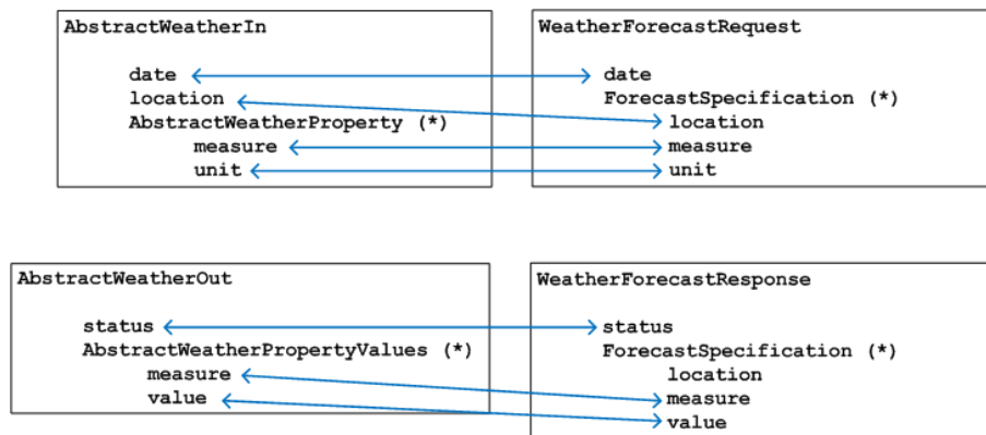
Figure 2.5: Operation mappings for the weather service abstraction.
