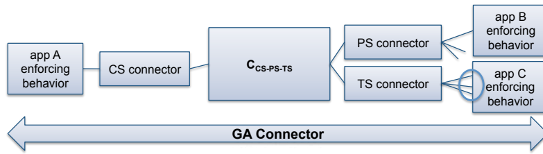
Figure 3.30: Tuning of the conversion method for GA
