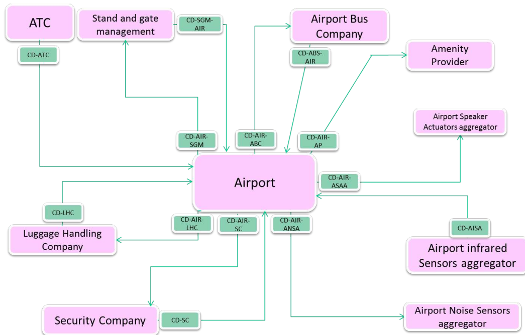
Figure 4.16: (a) Architecture of the airport use case
