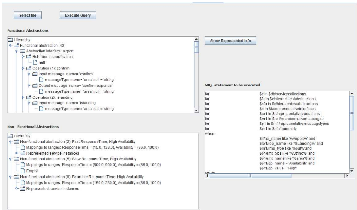
Figure 2.12: WSBQL execution in AoSBM.
