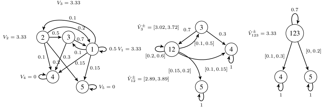
Figure 3: From left to right: the MDP M , the abstraction \alpha' , the abstraction \alpha . Edges are annotated with transition probabilities. The reward is: R(1) = R(2) = R(3) = 1 (= R(\{1, 2\}) = R(\{1, 2, 3\})) , and R(4) = R(5) = 0 .
