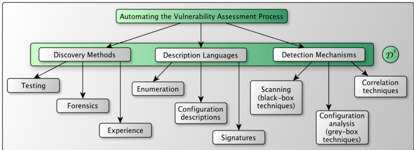
Fig. 5: Automated vulnerability assessment classification
