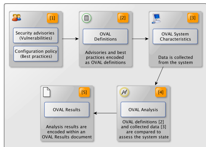
Fig. 7: OVAL-based vulnerability assessment [43]
