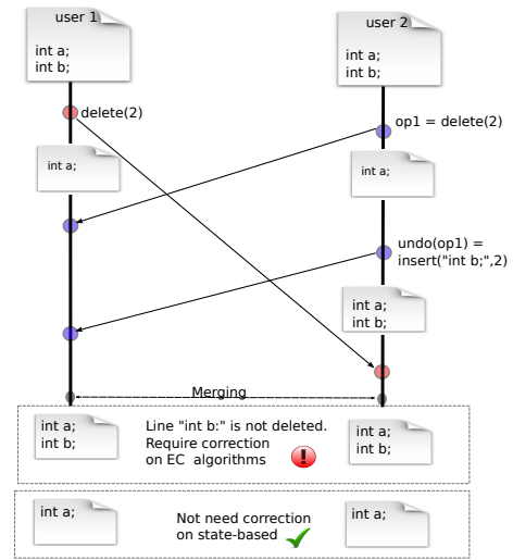
Figure. 5: undo/redo operation
