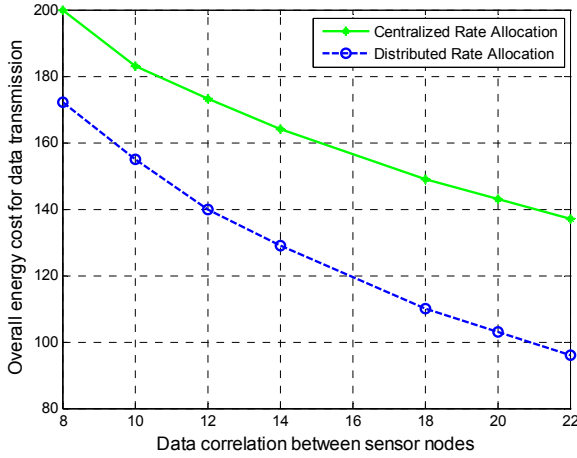
Fig.1 Overall energy cost in the network.
