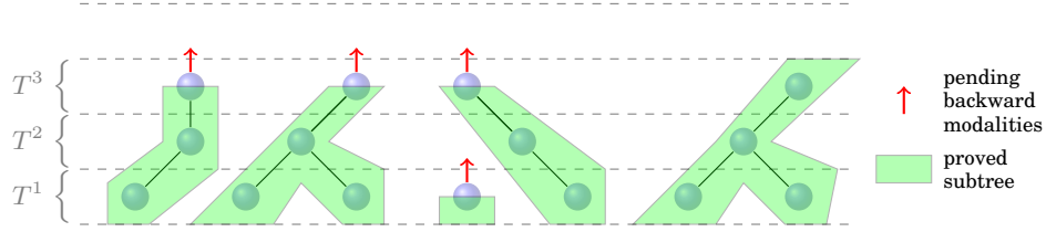
Fig. 7. Algorithm's principle: progressive bottom-up reasoning.
