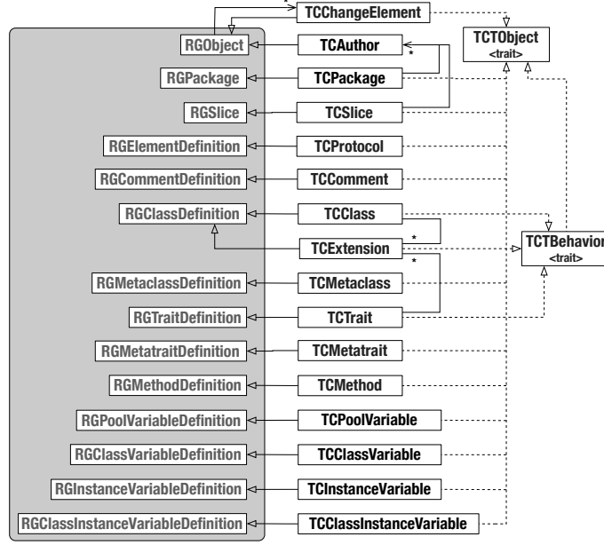
Figure 14: Torch change meta-model – Key classes.
