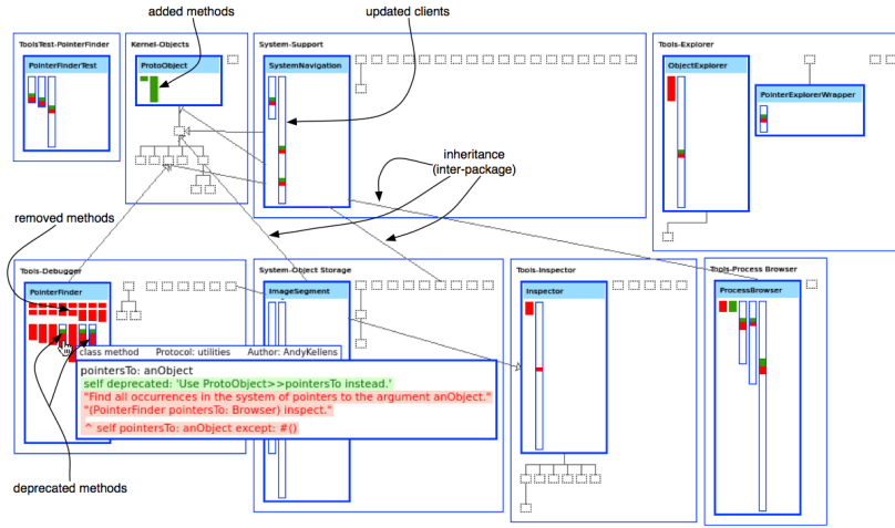
Figure 8: Removing the feature PointerFinder and deprecating its API: its functionality was substituted by another tool.
