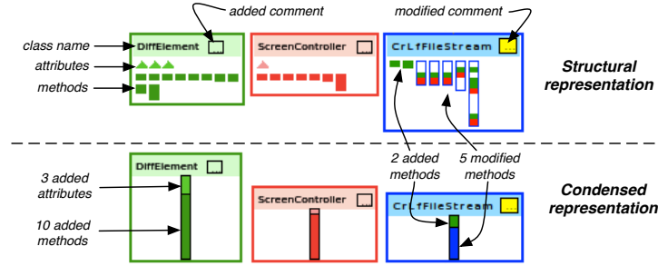
Figure 3: Structural and condensed visual representation of classes.
