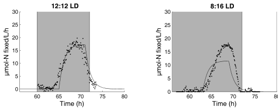
Fig. 2. Simulated (continuous line) and measured (dots) nitrogenase activity under the 12:12 LD and 8:16 LD light regimes, during 24 hours. White and grey backgrounds represent the light and dark periods, respectively.
