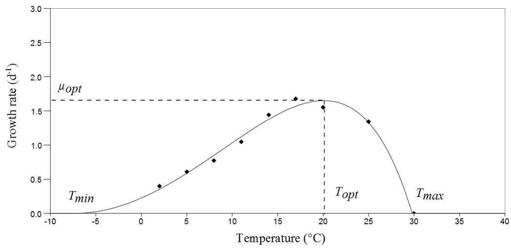
Figure 3. Experimental growth rate for Asterionella formosa (Butterwick et al., 2005) (◆) compared to CTMI predictions (curve) as a function of temperature (from Bernard and Rémond, 2012).
