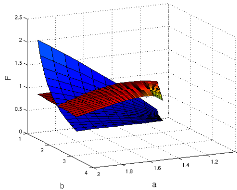
Figure 5: Probabilities P_{00 \rightarrow 10} (red surface) and P_{11 \rightarrow 10} (blue surface), as a function of a and b , for c = 0.5 .
