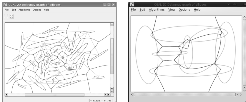
Figure 1: Left: Voronoi diagram and Delaunay graph of 26 ellipses; Right: Voronoi diagram of 7 intersecting ellipses
