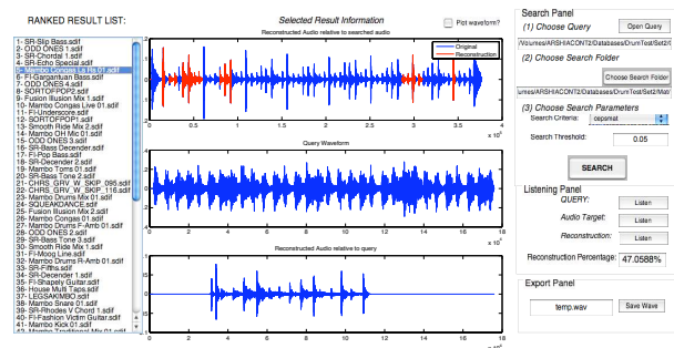
Figure 2. GUI for Audio Query over an Audio Database
