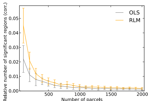
Figure 4. Percentage of parcels significantly associated with a non-null effect of the SNP \times Stressful\ Life\ Events\ (SLE) interaction, according to standard and robust regression. The latter always uncover more significant associations, which makes it a good candidate for a combined use with Randomized Parcellations Based Inference.
