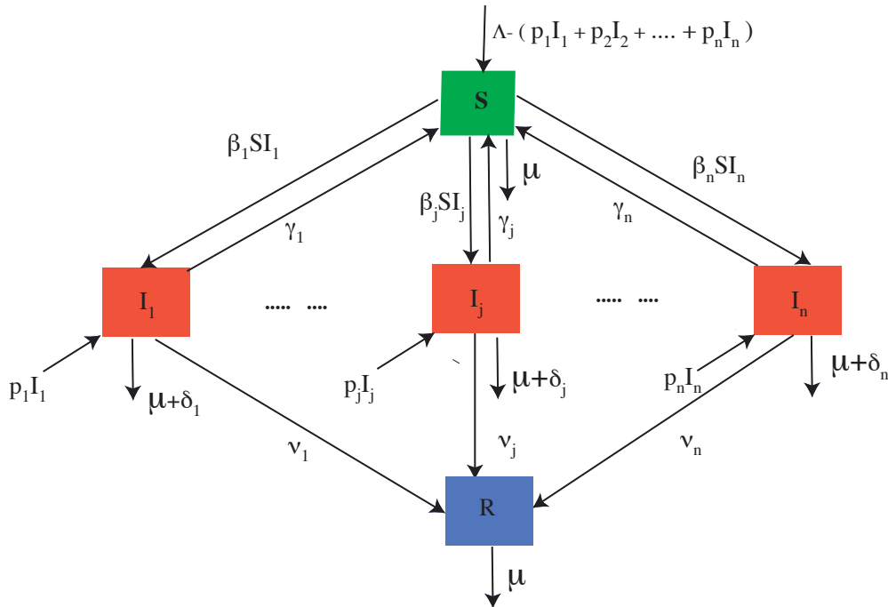
Figure 2: A SIR model with n strains
