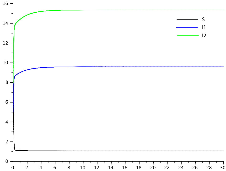
Figure 5: Non generic case: An SIS model with 2 coexisting strains. For the initial condition (S(0), I_1(0), I_2(0)) = (10, 5, 8) , this figure shows that the system (1) towards the equilibrium \bar{S} \approx 1.0612245 , \bar{I}_1 \approx 9.5965706 and \bar{I}_2 \approx 15.354513 . Obviously, the relation (9) holds: \Lambda - (\mu + \delta_1)\bar{I}_1 - (\mu + \delta_2)\bar{I}_2 - \mu\bar{S} \approx 0 .
