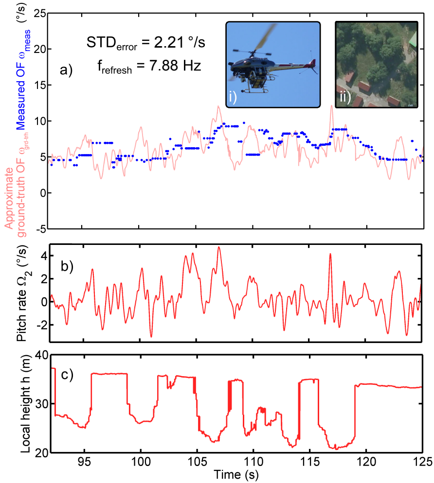
Fig. 7 Low-speed visual motion sensor and flight data sensed on-board the ReSSAC UAV. (a) Approximate ground-truth optic flow (see (17)) (red) and measured optic flow \omega_{\text{meas}} = \Delta\varphi/\Delta t (blue dots). Despite the strong variations mainly due to vibrations, the low-speed visual motion sensor’s output closely matched the approximate ground-truth optic flow, giving a standard deviation of 2.21^\circ/\text{s} and a refresh rate of 7.88 \text{ Hz} . The effects of strong variations in the local height due to the successive trees and houses are directly reflected in the low-speed VMS measurement signal. (i) ReSSAC unmanned helicopter in-flight (ii) Aerial view of the flight environment obtained on http://geoportail.fr . (b) Pitch angular rate of ReSSAC as measured by the IMU. (c) Local ground height measured by combining GPS data and previously mapped LIDAR data. The nominal height was around 40 m. But due to the variable relief, the local height often changed suddenly by 15 meters.
