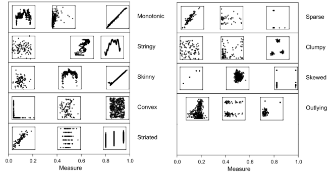
Figure 2: Nine scagnostics measures from [16].
