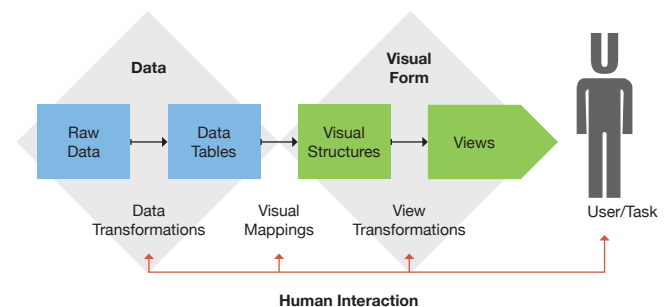
Fig. 2. The Information Visualization Reference Model according to [2]. On the top of the pipeline, data is adapted to be visualized and converted into an image through a visual mapping and a view. On the bottom, user interaction allows controlling all the stages of the pipeline with immediate feedback.
