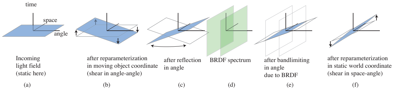
Fig. 3: Frequency analysis of BRDF shading for a rotating glossy plane. We model shading as a static operation (c-e) in the coordinate system of the moving receiver. The changes of coordinates occur in (b) and (f). The spectrum of the static incoming light (a) has a temporal component (b) in the coordinate system of the moving receiver.
