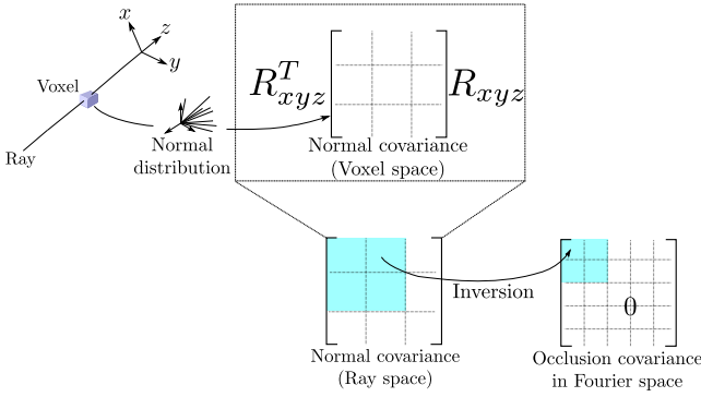
Fig. 8: We use a voxel grid to handle occlusion, and store normal distributions at each voxel. This information is used to estimate the local 2D spectrum of obstacles as they partially occlude the local light field at points along the central light ray. The stored covariance matrix (of the local normal distribution) is first rotated to align it with the local frame of the ray and then the appropriate 2D sub-matrix (corresponding to the tangent frame of the ray) is projected to the XY plane of the local light field.
