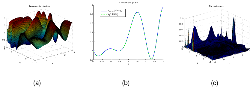
Figure 1. Example 1: V_2(x, y) = \sin(\frac{1}{2}x^2 + \frac{1}{4}y^2 + 3) \cos(2x + 1 - e^y) + 1 . (a) V_{2,h,\gamma,0}(x_i, y_j) . (b) V_2(-0.62, y_j) , V_{2,h,\gamma,0}(-0.62, y_j) with y_j = -1, -0.98, \dots, 3 . (c) The relative error between the real function and its estimation.
