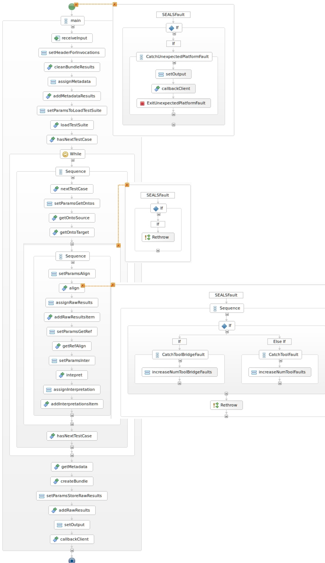
Figure A.1: BPEL workflow for the evaluation of ontology matching tools.
