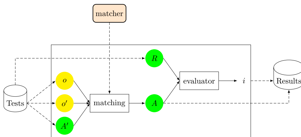
Figure 2.2: Extended evaluation workflow with alternative input alignment.
