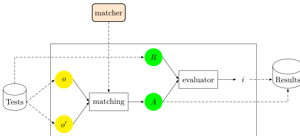
Figure 2.1: Basic evaluation workflow.
