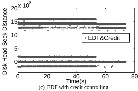
Figure 8: Disk head seek distance under Flubber , base CFQ, CFQ with priority settings, and EDF with credit controlling, when running two-classes of Read applications
