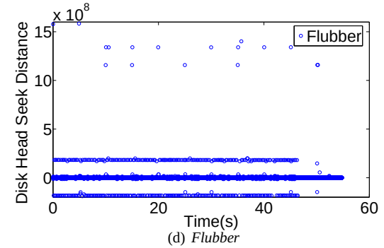
Figure 8: Disk head seek distance under Flubber , base CFQ, CFQ with priority settings, and EDF with credit controlling, when running two-classes of Read applications
