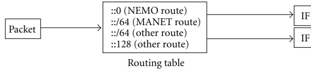
FIGURE 5: Classic routing. A single routing table is used, and packets are forwarded along the route with the longest matching prefix.
