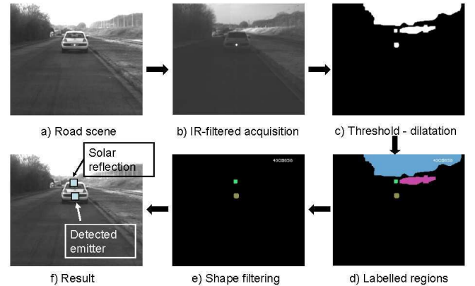
Fig. 5. Low-level Image Analysis.
