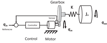
Fig. 2. model of robot joint with compliance
