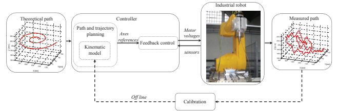
Fig. 1. functional chain of industrial robots
