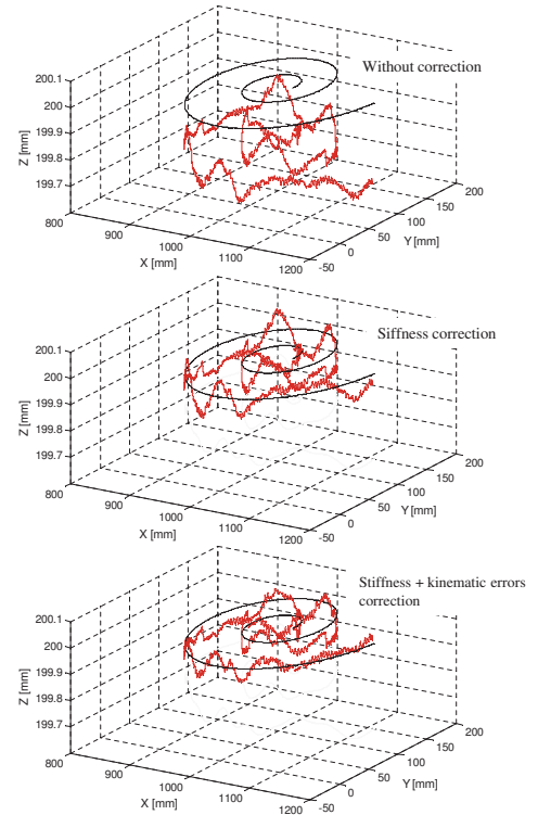
Fig. 13. measured trajectories without and with correction
