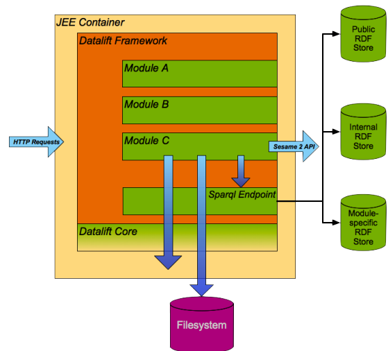
Figure 2: Datalift Architecture
