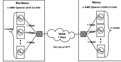
Figure 4. Experimental testbed.
