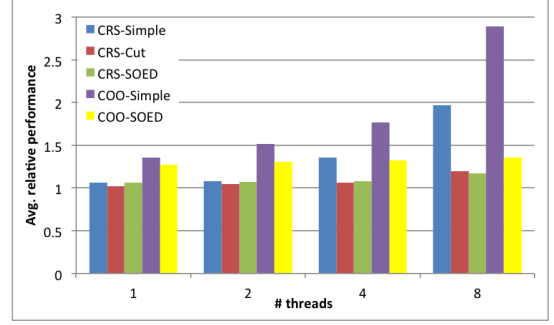
Figure 6. Average relative performances of parallel scaling algorithms on the AMD-based architecture. The relative performance of each algorithm on a particular problem is computed by dividing the average execution time of the algorithm by the best average time for the same problem.
