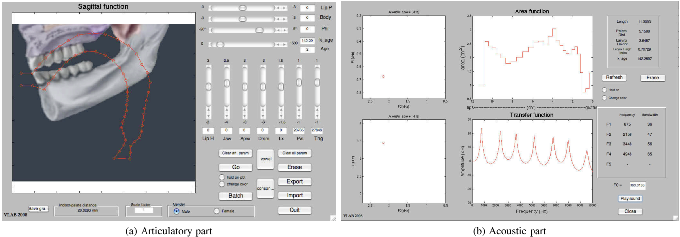
Fig. 3. VLAM processing flow. Articular part: a vocal tract shape is generated from the seven articular commands; Acoustic part: from the area function (top right), the spectrum of the vocal tract transfer function is computed (bottom right) leading to formant values positioned in the (F_1, F_2) and (F_2, F_3) spaces (left).
