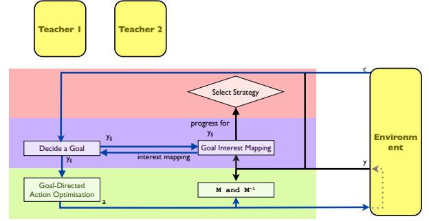
Figure 1: Data Flow under the Intrinsic Motivation strategy
