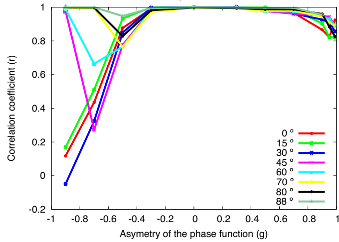
(b) Input angle \theta_i ( \alpha = 0.99, \eta = 1 )
