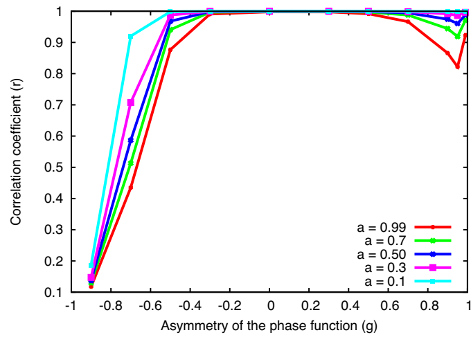
(a) Albedo \alpha ( \eta = 1, \theta_i = 0 )
