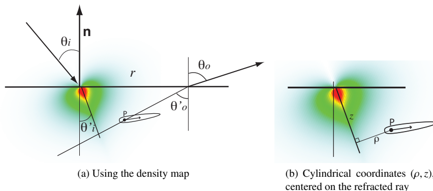
Figure 4: We compute the density of two scatter events around the scattered ray inside the material, along with average direction. At rendering time, we find the contribution at sample point P using the density, average direction and phase function.
