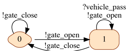
Figure 7. Requirement R_{g.1} specified as an i/o-automaton. Prefix “?” indicates an input and prefix “!” indicates an output.
