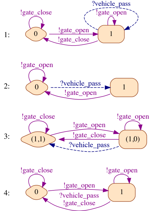
Figure 9. Translating the assumptions of \mathbf{gate} as a Modal Interface A_{\mathbf{gate}} using Rules 2. 1: translation of R_{g,1} ; 2: translation of R_{g,2} ; 3: the resulting conjunction; 4: the final result after applying rule R_3^A and renaming the states.
