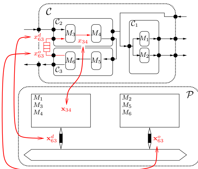
Figure 6. Mapping the application to the execution platform as \mathcal{C} \wedge \mathcal{P} .
