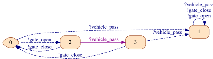
Figure 10. Chapter gate of the top-level requirements document translated into a Modal Interface \mathcal{C}_{\text{gate}} .
