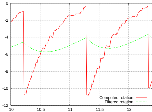
Figure 9: Simulation experiment: steering angle (in degrees) in the first turn of the path with respect to the time (in second). The computed steering angle in red shows two exponential decreasement corresponding to two visual servoing tasks, the filtered steering angle is in green.
