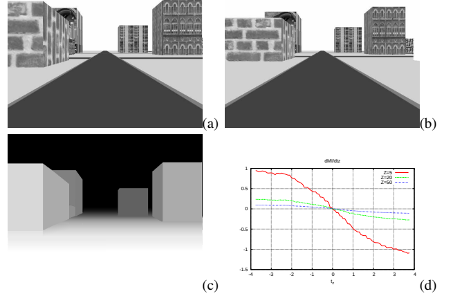
Figure 7: Translation estimation between the current and desired image. (a) Desired image, (b) acquired image with a 4 meter translation, (c) scene depth and (d) derivative of mutual information with respect to the translation along the z axis (in meters) with various fixed scene's depth Z .
