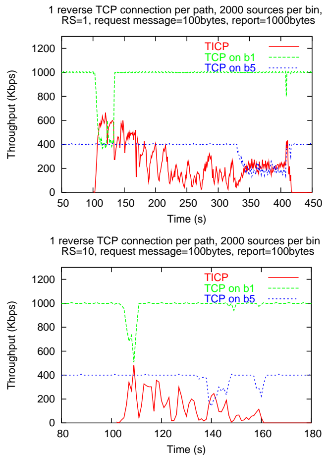
Fig. 9. One TICIP session and one long-lived TCP connection per path, congestion in the reverse direction, better TCP-friendliness
