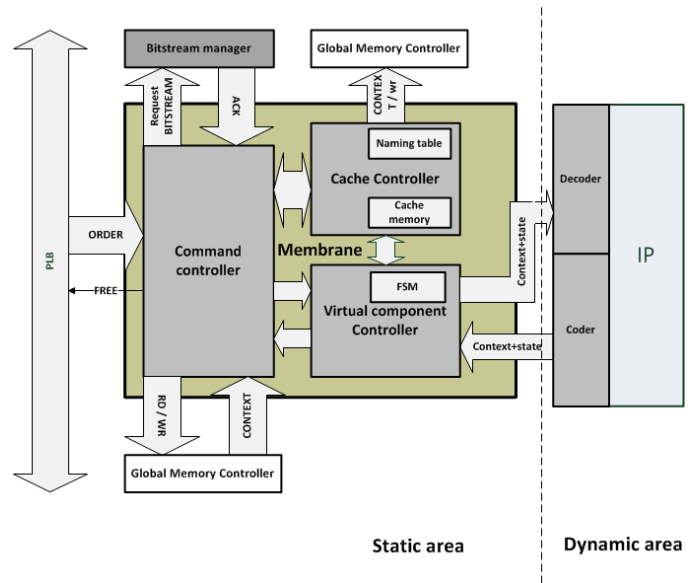
Fig. 3. Membranes architecture and interconnection
