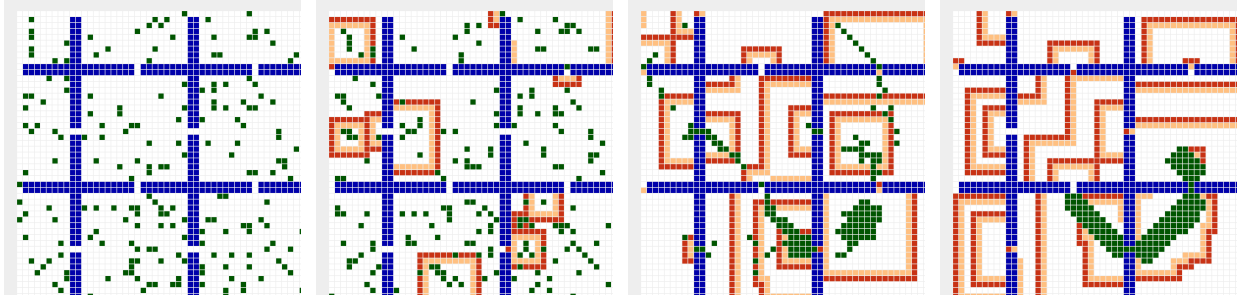
Figure 3: Agent aggregation in the presence of obstacles, for times t=0, 20, 100 and 700 . Agents are shown in green, obstacles in blue, neutral cells in white and excited cells with red.
