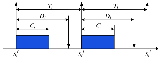
Figure 1. Model for non-preemptive strict periodic task \tau_i(S_i^0, C_i, D_i, T_i)
