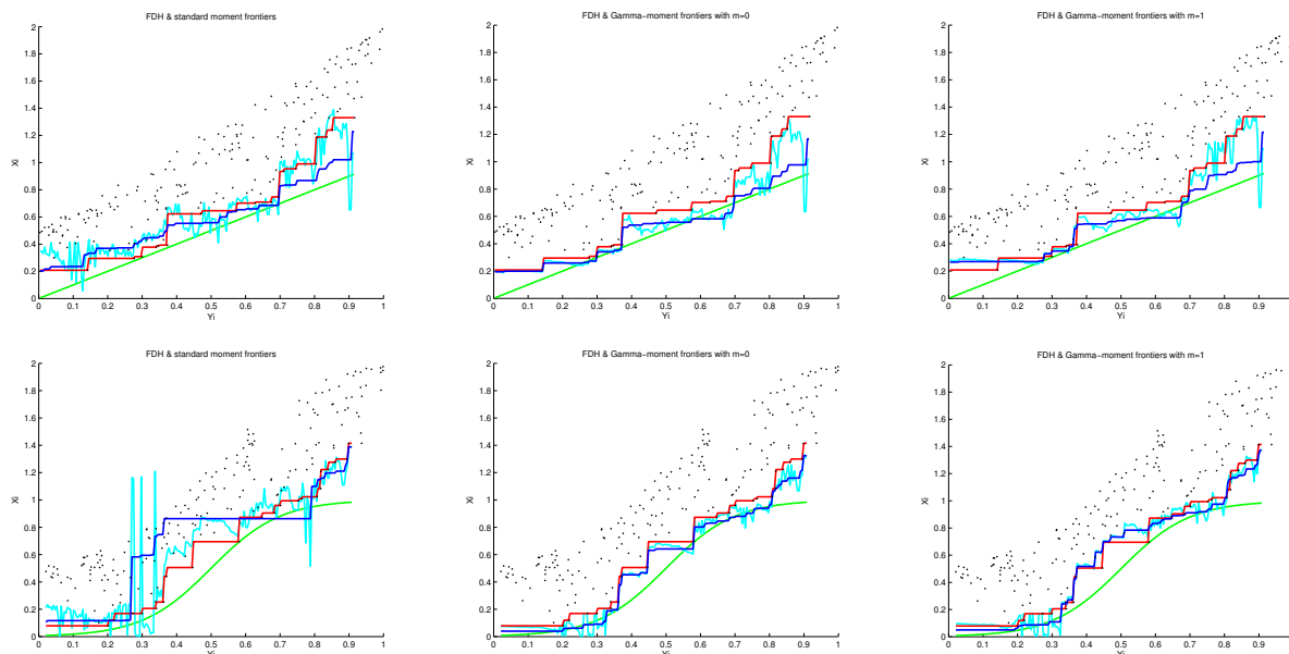
Figure 2: Results for \gamma_y > -1/2 and n = 200 using the bootstrap quantity (16) in step 2.
