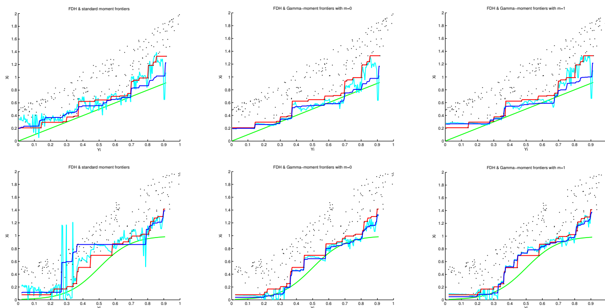
Figure 2: Results for \gamma_y > -1/2 and n = 200 using the bootstrap quantity (16) in step 2.
