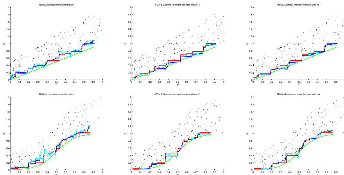
Figure 1: Results for \gamma_y = -1/2 and n = 200 using the bootstrap quantity (16) in step 2.
