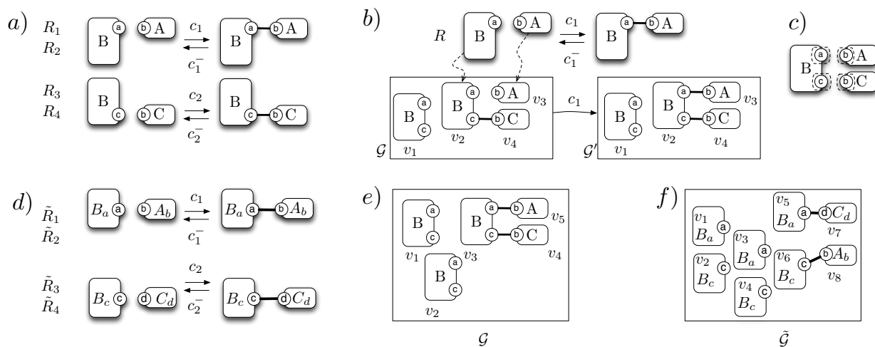
Figure 1: Illustration. a) A rule set over the set of node types \mathcal{A} ; b) Rule application: Rule R can be applied to a reaction mixture \mathcal{G} via the embedding indicated by the dotted arrows. The result of the rule application is the reaction mixture \mathcal{G}' , and the corresponding rate is c . c) Annotation of the node types; d) The translation to a new set of node types \tilde{\mathcal{A}} ; e) An \mathcal{A} -reaction mixture; f) An \tilde{\mathcal{A}} -reaction mixture.
