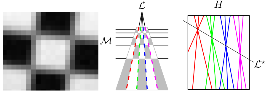
Fig. 3.1 Left: Example chequers from a ToF amplitude image. Note the variable appearance of the four junctions at this resolution, e.g. ‘ \times ’ at lower-left vs. ‘+’ at top-right. Middle: A perspective image of a calibration grid is represented by line-pencils \mathcal{L} and \mathcal{M} , which intersect at the \ell \times m = 20 internal vertices of this board. Strong image-gradients are detected along the dashed lines. Right: The Hough transform H of the image-points associated with \mathcal{L} . Each high-gradient point maps to a line, such that there is a pencil in H for each set of edge-points. The line \mathcal{L}^* , which passes through the \ell = 4 Hough-vertices, is the Hough representation of the image-pencil \mathcal{L} .
