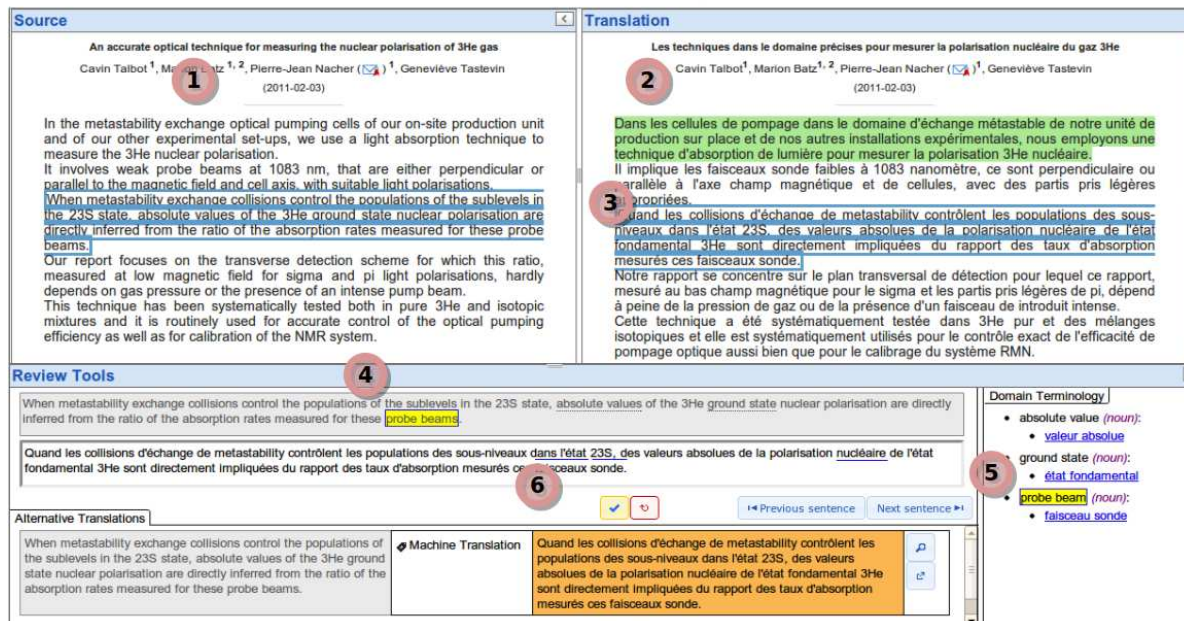
Figure 1: Translation and post-editing interface.
