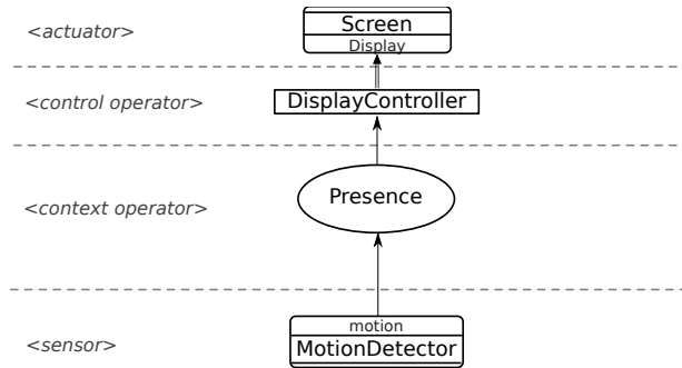
Figure 3: Graphical representation of the “HelloWorld” application design.
