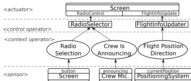
Figure 10: The flight entertainment system.
