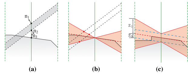
Figure 7: Ray refinement for transient edges. (a) A thin object intersection near the boundary of a pixel, which could be totally missed based on ray intersection points. (b) Uncertainty region for the third intersection point and approximation planes for the other two points. Intersections between the uncertainty region and the approximation planes indicate the existence of transient edges. (c) Surface uncertainty region with a narrow face.
