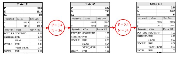
Figure 23: Representation of the situation where the person passes to the crouching posture and then returns to the standing posture in the hierarchy obtained for the learning context Position – Posture – SymbolicDistance .
