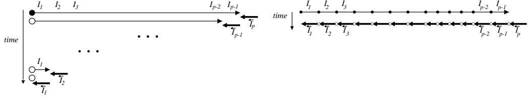
Figure 2: Data-flow reversal with Recompute-All approach ( left ) and Store-All approach ( right ). Big black dot represents storage of X_0 , big white dots are retrievals. Small black dots are values being recorded before overwriting. Small white dots are corresponding restorations.
