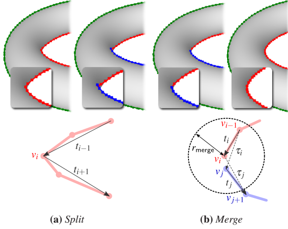
Figure 5: Split and merge operations modify snake connectivity. (a) When a snake bends too sharply around a corner it is split. (b) When two snakes abut smoothly they are joined.
