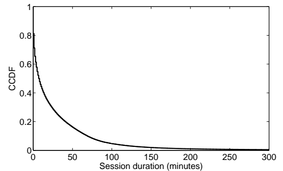
Fig. 4. Session duration derived from 60-minutes intersession threshold
