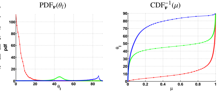
Fig. 9. Comparisons of the \text{PDF}_{\mathbf{v}} and the inverse \text{CDF}_{\mathbf{v}}^{-1} for nickel material. The measured inverse CDF curves traced in red for \theta_v = 0^\circ , in green for \theta_v = 45^\circ , and in blue for \theta_v = 85^\circ , are always simpler than the ones for the PDF.
